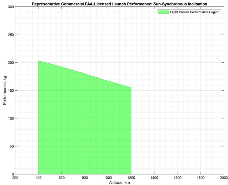
Figure 1b: Sun-Synchronous Inclination Constraining Performance Curves
