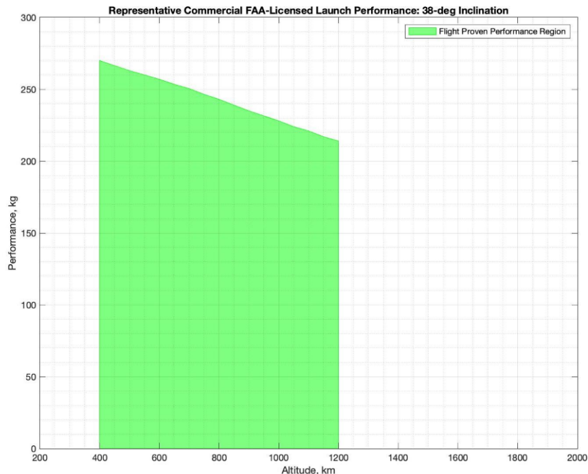
Figure 1a: 38 Degree Inclination Constraining Performance Curves
